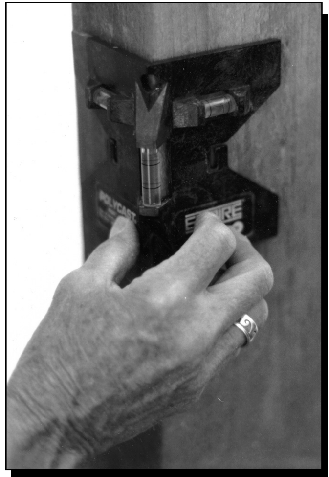
Figure 76—Post level.
