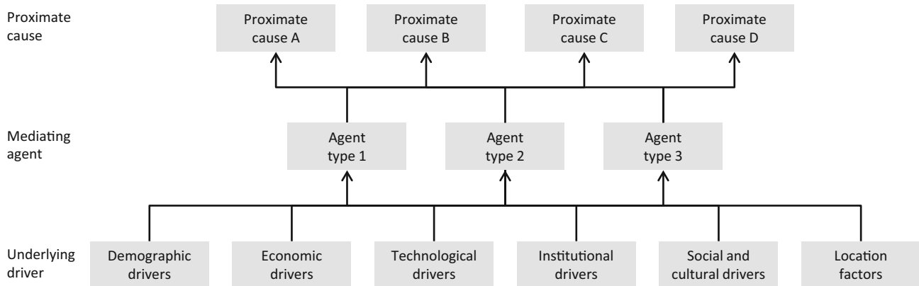
Fig. 2 Two conceptually different models for drivers of land use change: a Proximate causes and underlying drivers; b Explicitly considering agents as moderators between underlying drivers and proximate causes
